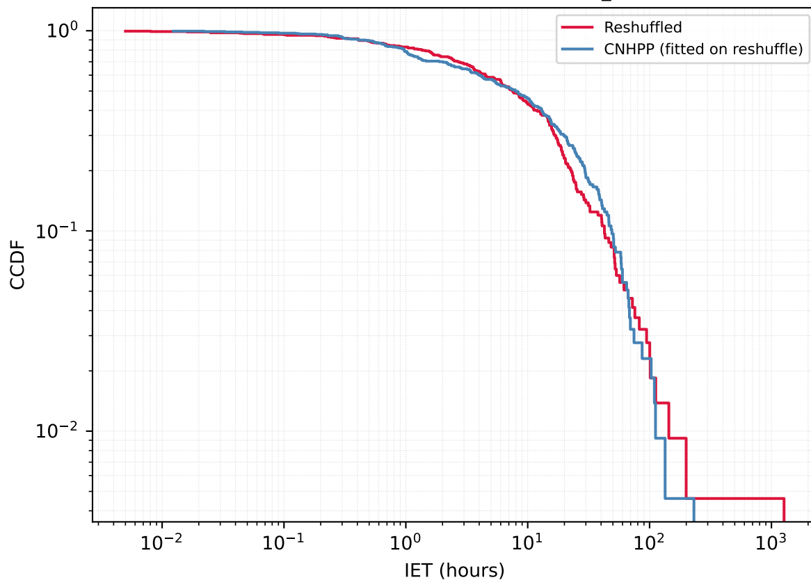
User 5657126860 - Reshuffled vs CNHPP A_{\text{fit}}=0.3909
